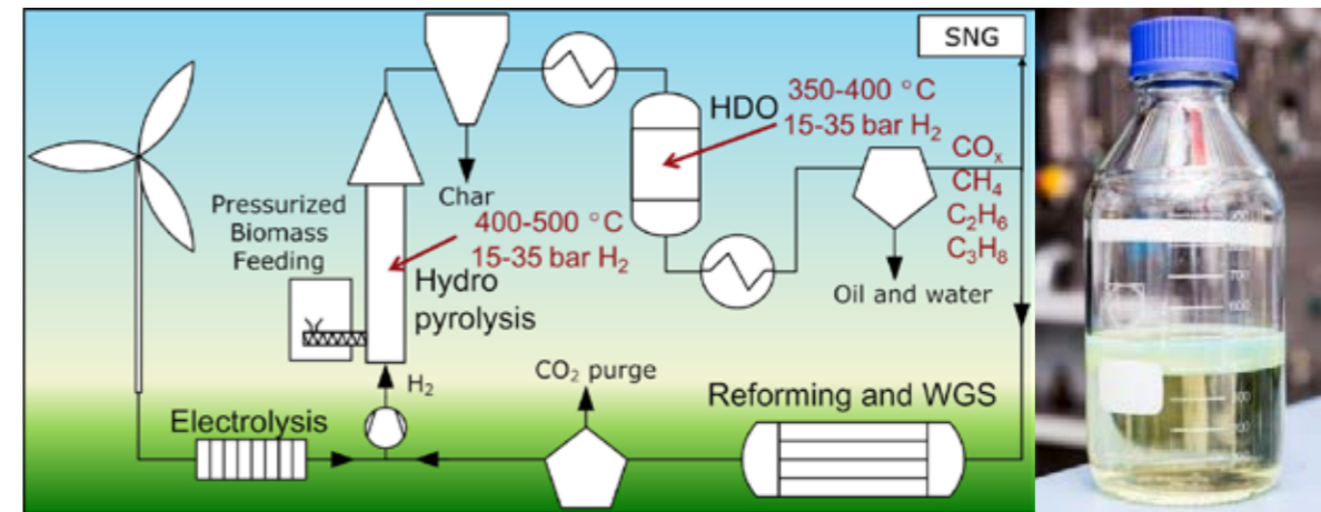
Figure 7. Proposed catalytic hydropyrolysis process diagram and example of hydropyrolysis liquids formed in the laboratory of DTU Chemical Engineering, showing the phase separation of oil (top) and water (bottom).
