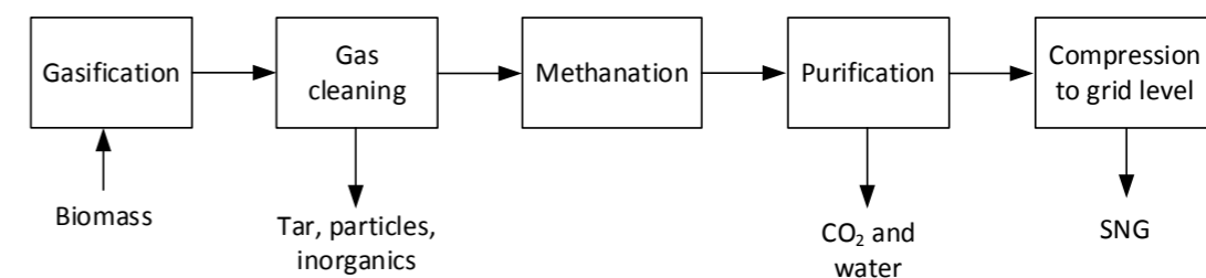
Figure 3. Typical flow diagram for SNG synthesis from product gas
