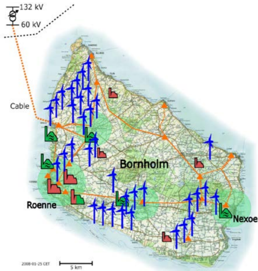
Figure 6. Map of Test Zone Bornholm, with power system and 60kV connection to Sweden
