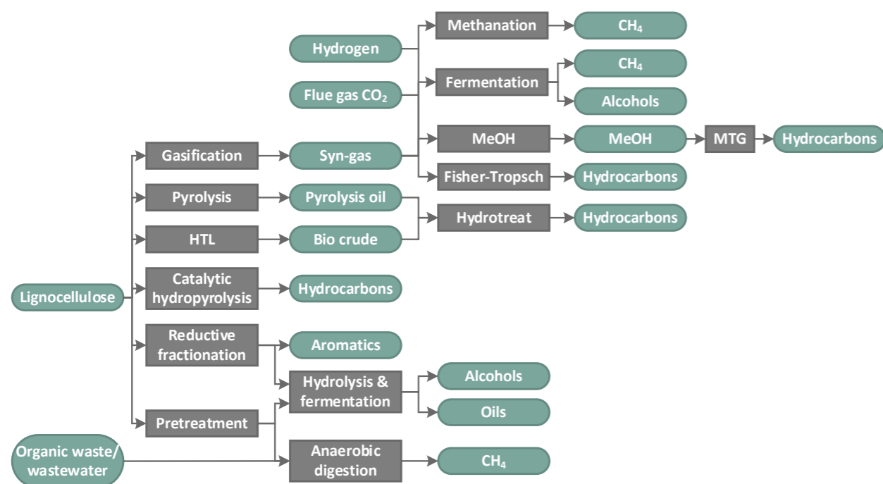
Figure 1. Main routes from lignocellulosic biomass, liquid organic waste and industrial flue gases to liquid and gaseous fuels suitable for the transport sector. The conversion processes are illustrated in the rectangles, while the rounded shapes indicate compounds or other substances. HTL: hydrothermal liquefaction, MeOH: methanol (synthesis), MTG: methanol to gasoline
