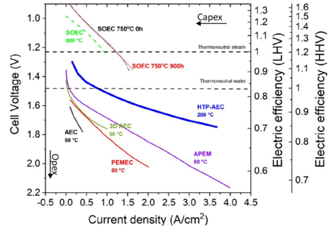
Figure 2. Cell voltage versus current densities for various types of electrolysis technologies applicable for the production of hydrogen by water/steam splitting. Right-hand scales illustrate the achievable efficiencies
