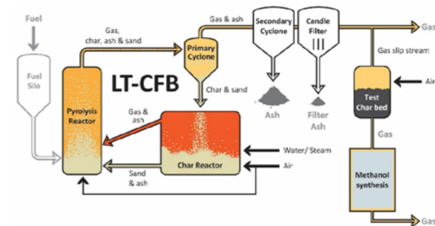
Figure 5. LT-CFB gasifier coupled to a partial oxidation chamber, char bed and methanol synthesis
