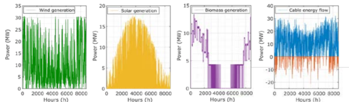
Figure 7. Local power generation over the year and exchange via the cable to Sweden
