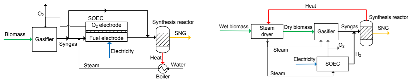
Figure 4. Right: wet biomass to SNG by integration of steam drying, gasification and SOEC. Left: dry biomass to SNG by gasification coupled with pressurized SOEC with internal methanation
