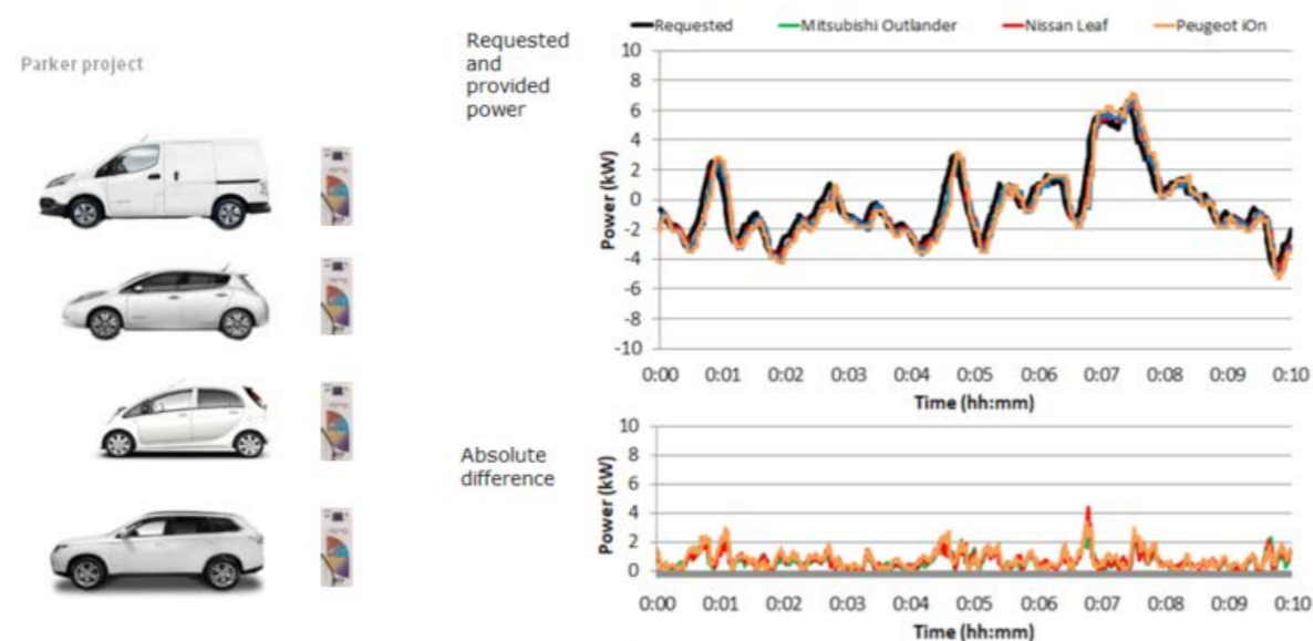
Figure 9b. Frequency regulation tested across several EV brands [4;19]
