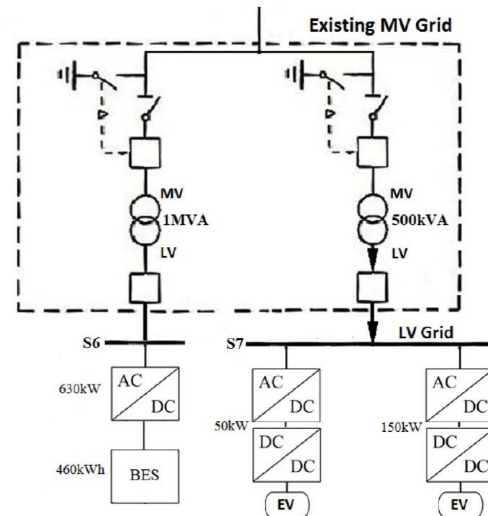
Figure 4. Illustration of fast charger in EnergyLab Nordhavn (courtesy Nerve Smart Systems Aps). The diagram shows how the BESS (BES) and the two fast chargers are connected to the 10kV electric grid through 0.4/10kV transformers [14].
